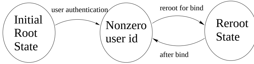
Figure 4. State diagram of the wu-ftp daemon
